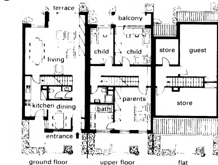
9 Terraced houses with transverse stairs
